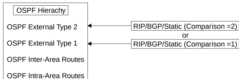
Figure 17-2. OSPF Routing Hierarchy
