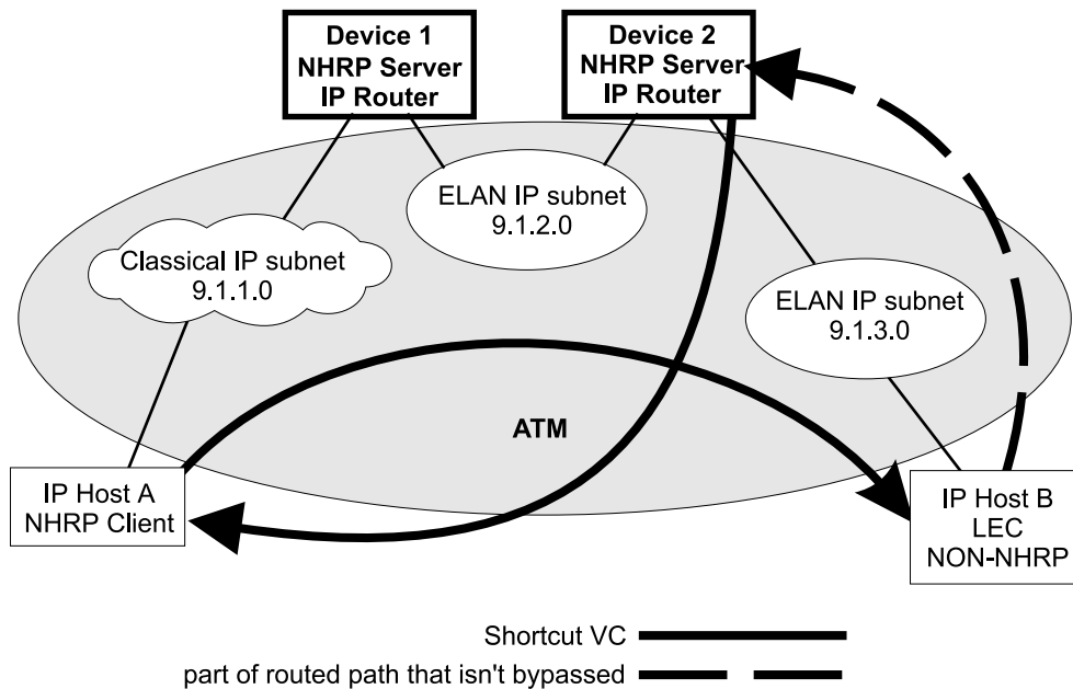
Figure 30-6. NHRP in a Mixed Classical IP and ELAN Environment
