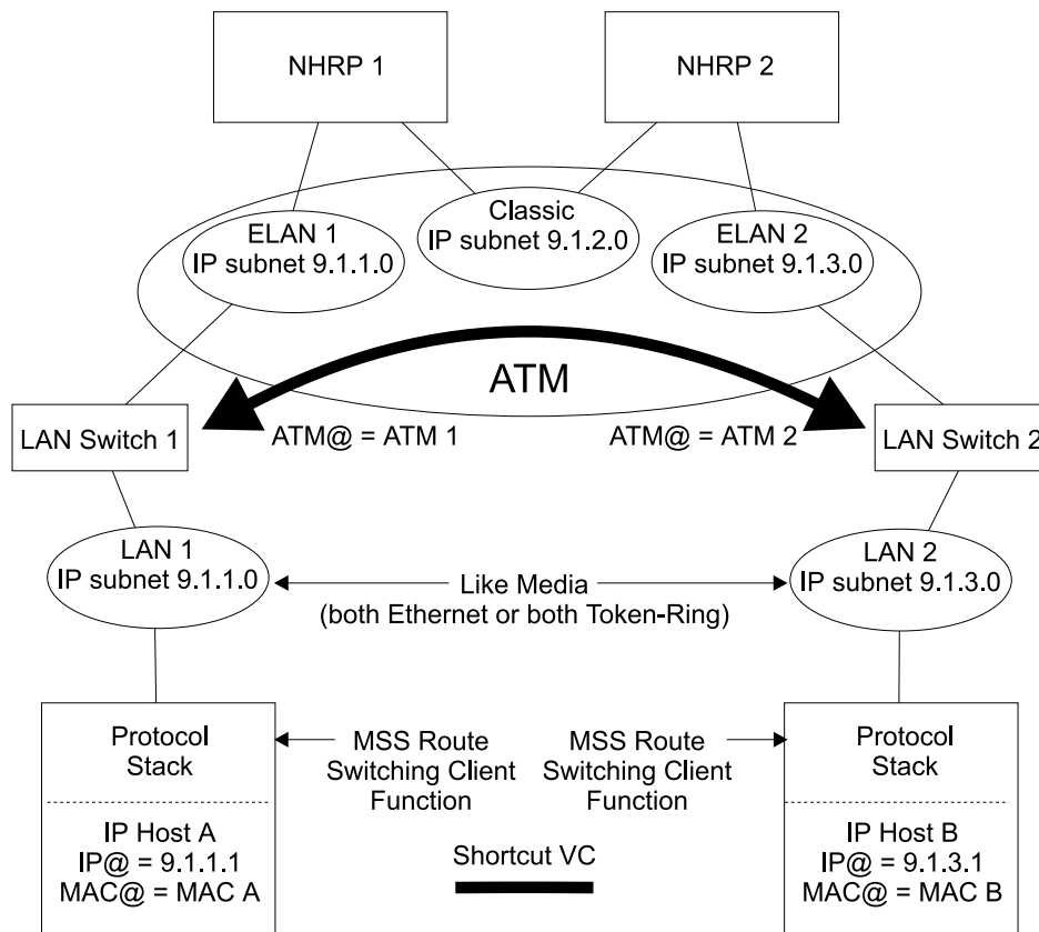
Figure 30-10. Route Switching in Both Directions
