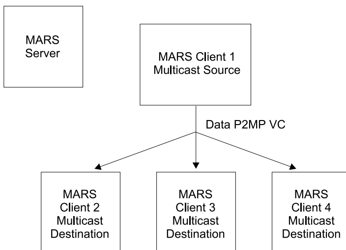
Figure 26-2. VC Mesh
