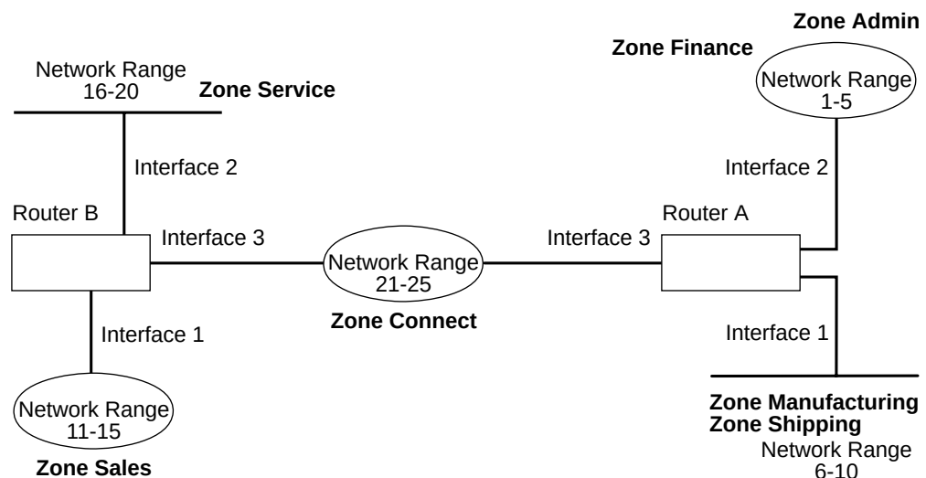
Figure 32-2. Example of Network Filtering.
