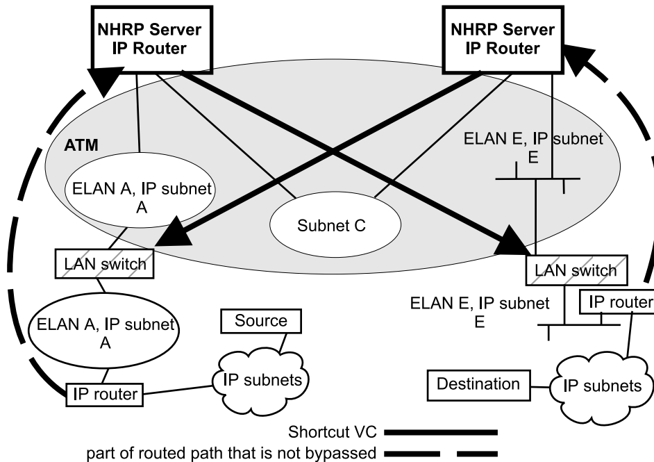
Figure 30-7. NHRP to an Egress Router
