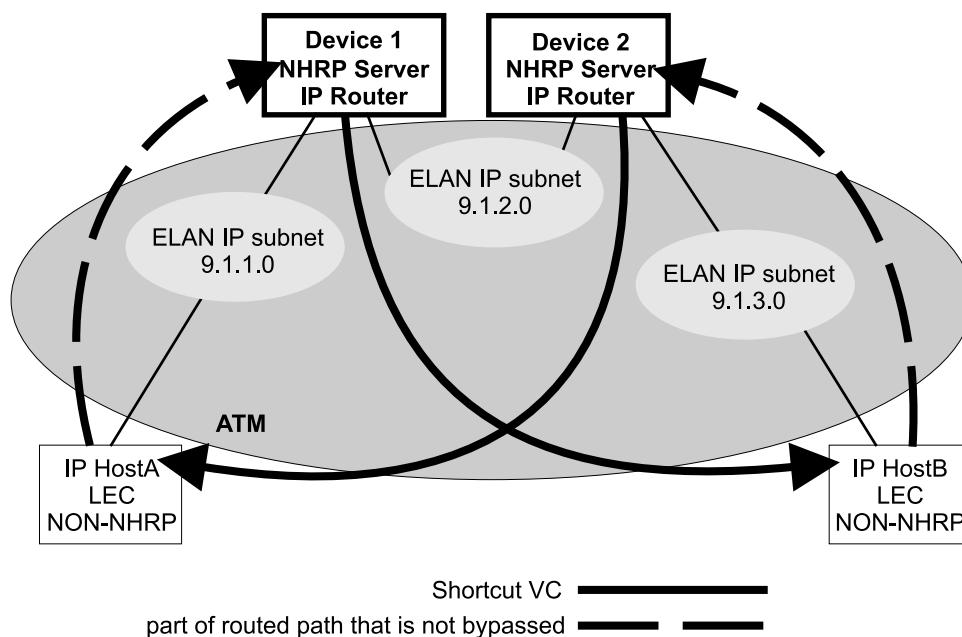
Figure 30-4. NHRP in an ELAN Environment
