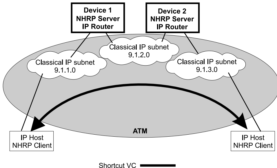
Figure 30-2. NHRP in a Classic IP Environment
