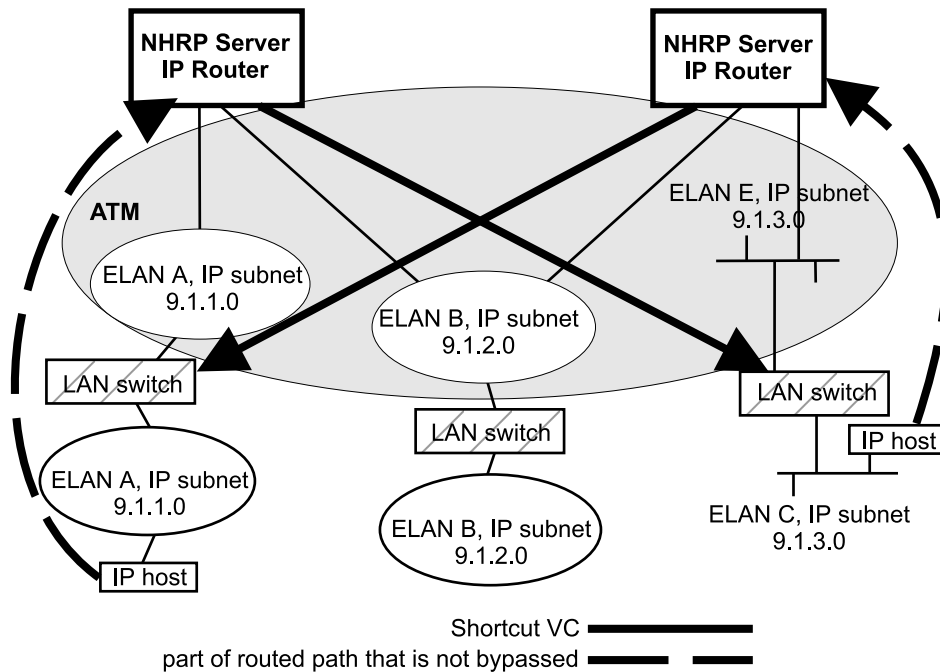
Figure 30-5. NHRP in an ELAN Environment with LAN Switches
