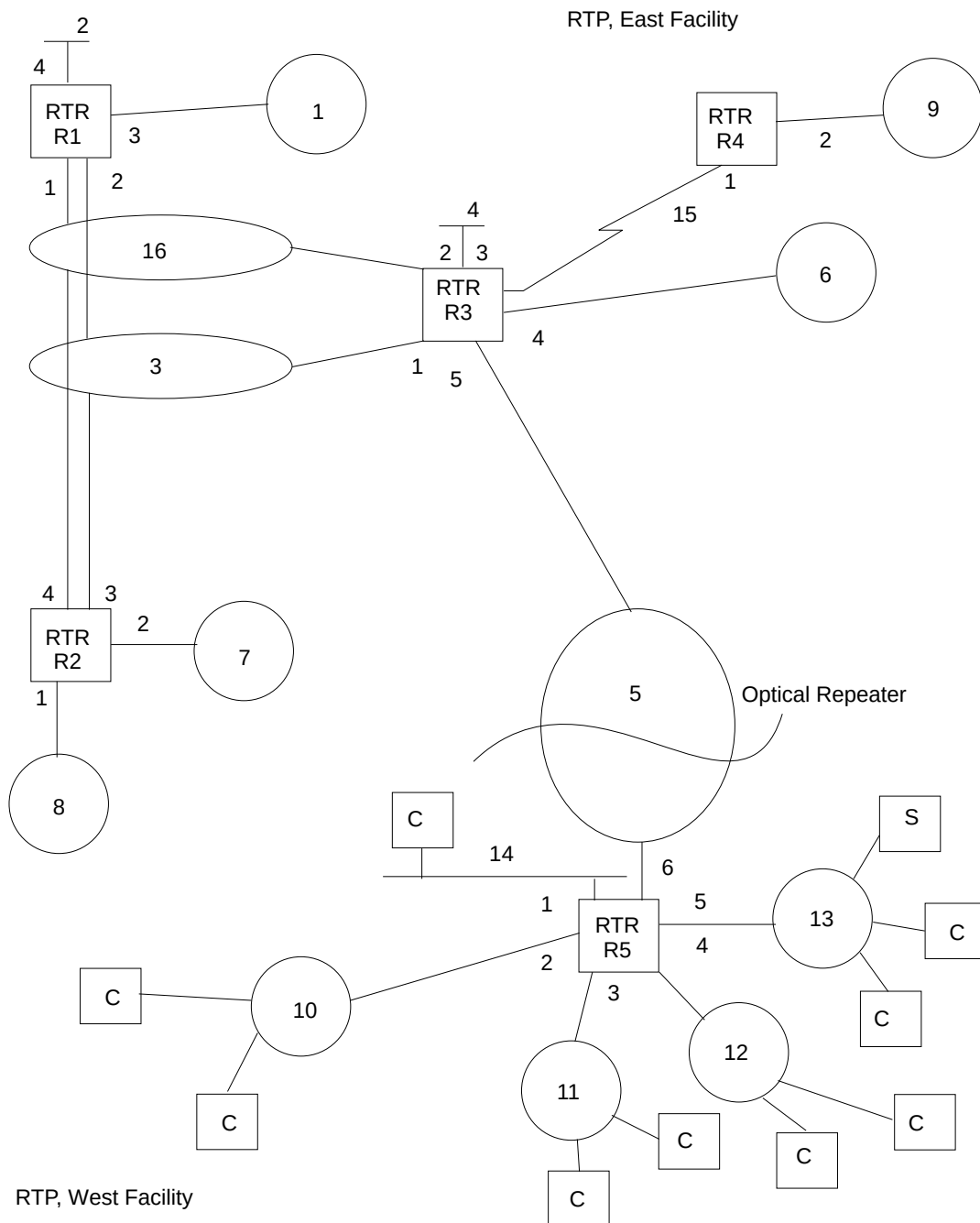
Figure 21-1. Sample IPX Network
