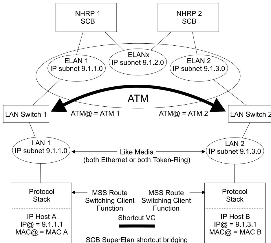
Figure 30-12. Route Switching in a SuperELAN Environment
