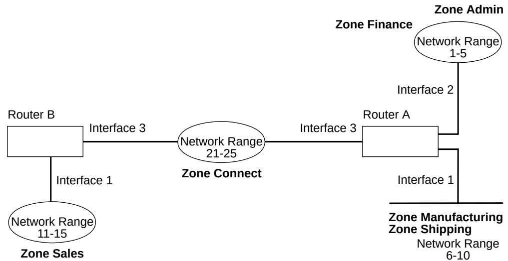
Figure 32-1. Example of Zone Filtering
