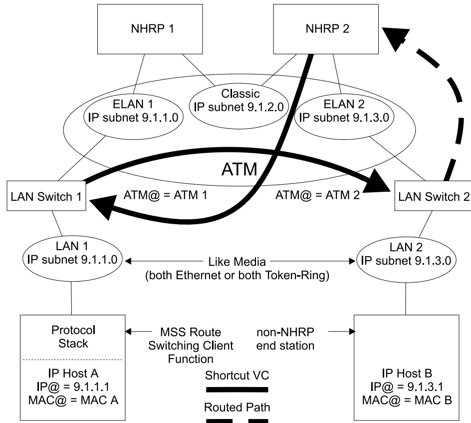
Figure 30-11. Route Switching in One Direction
