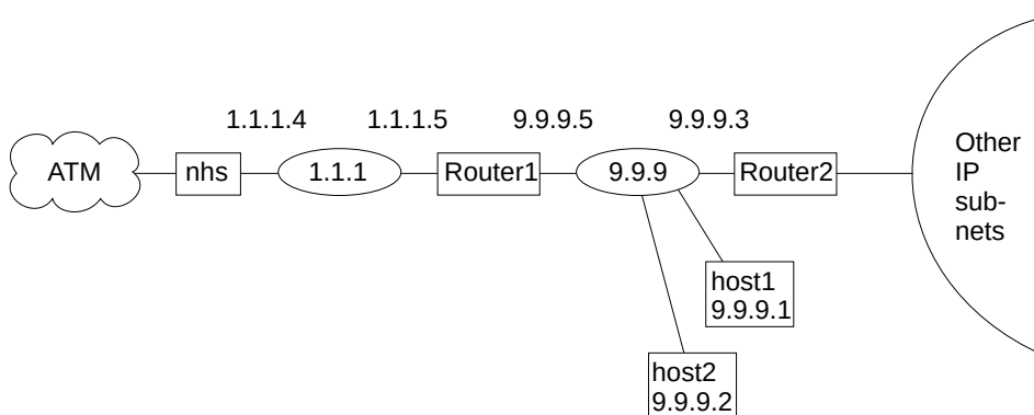
Figure 30-8. Using Disallowed Router-to-Router Shortcuts
