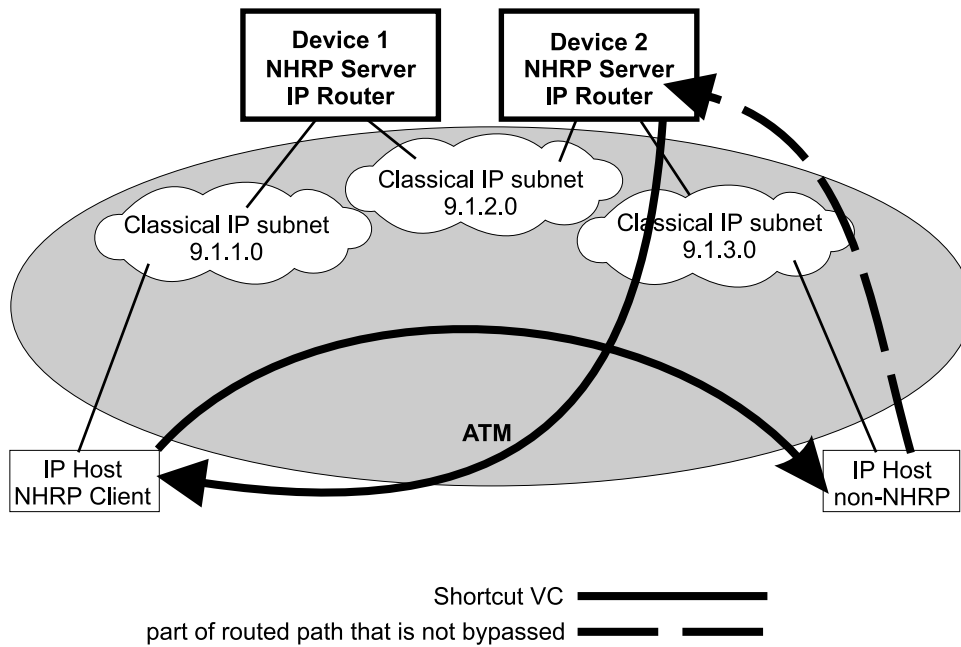
Figure 30-3. NHRP in a Classic IP Environment with non-NHRP Device
